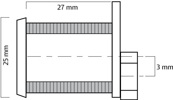
Cylinder Dimensions
