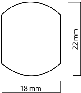
Cylinder Housing Cut-out Dimensions
